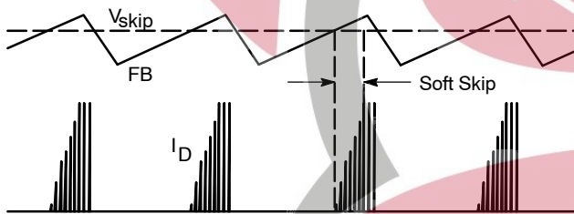
Figure 36. Soft-Skip Operation
