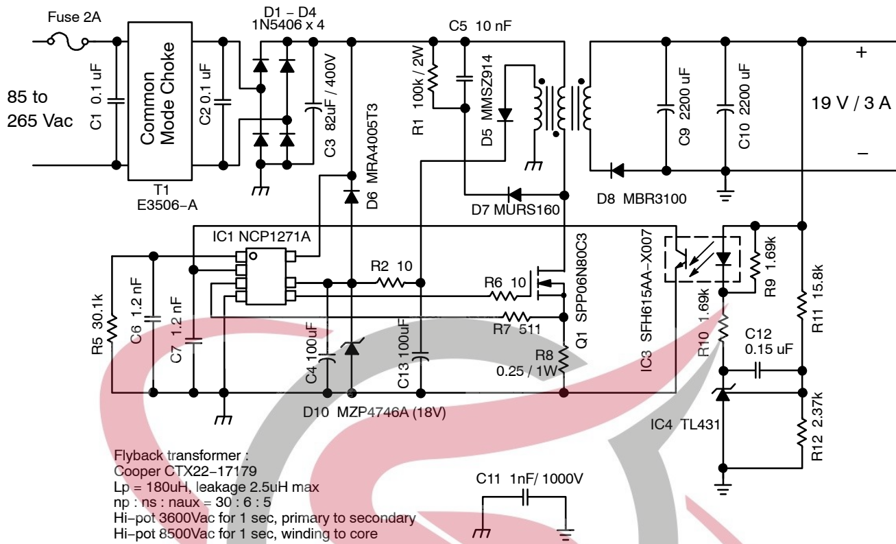
Figure 42. 57 W Example Circuit Using NCP1271
